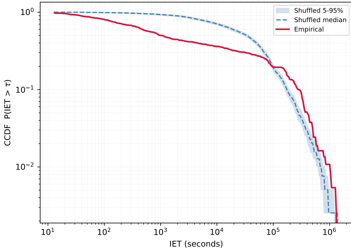
User 412633448 - Empirical vs Reshuffled | KS=0.461 p=0.000
